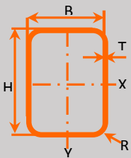
Rectangular Hollow Sections Size Range
